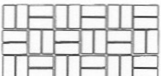
Large Blockweave Brick Size 125mm x 265mm
